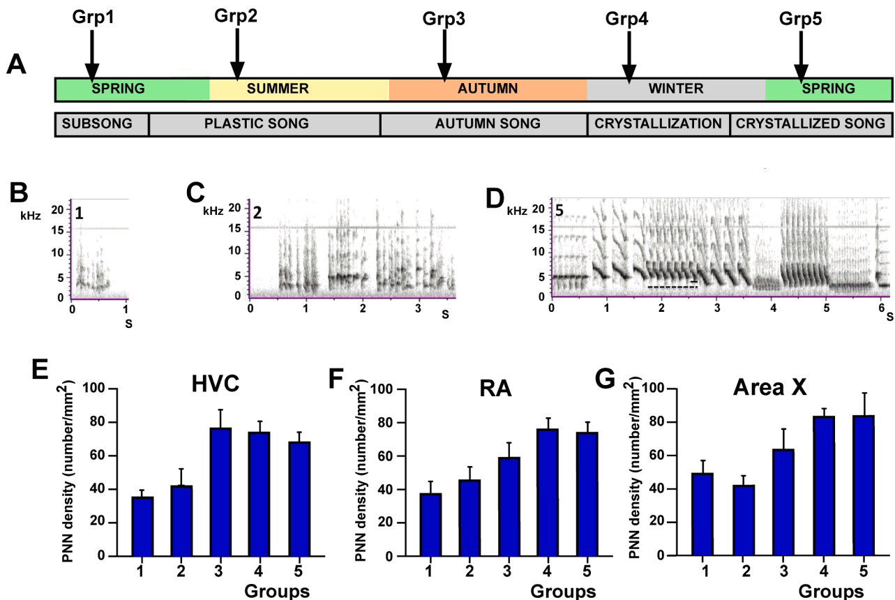
Fig. 2. Perineuronal nets and song development during ontogeny in male canaries. A. Schematic representation of song development in male canaries during their first year of life and distribution in time of the 5 experimental groups (Grp 1 to 5). B-D. Examples of spectrograms illustrating the 3 main stages of song development, subsong (B), plastic song (C) and crystallized song (D). E-G. Changes in PNN density (numbers /mm 2 ) during ontogeny in three song control nuclei in male canaries. All data are means \pm SEM of 7 to 10 data points per age. Redrawn and rearranged from data in (Cornez et al., 2020b).
